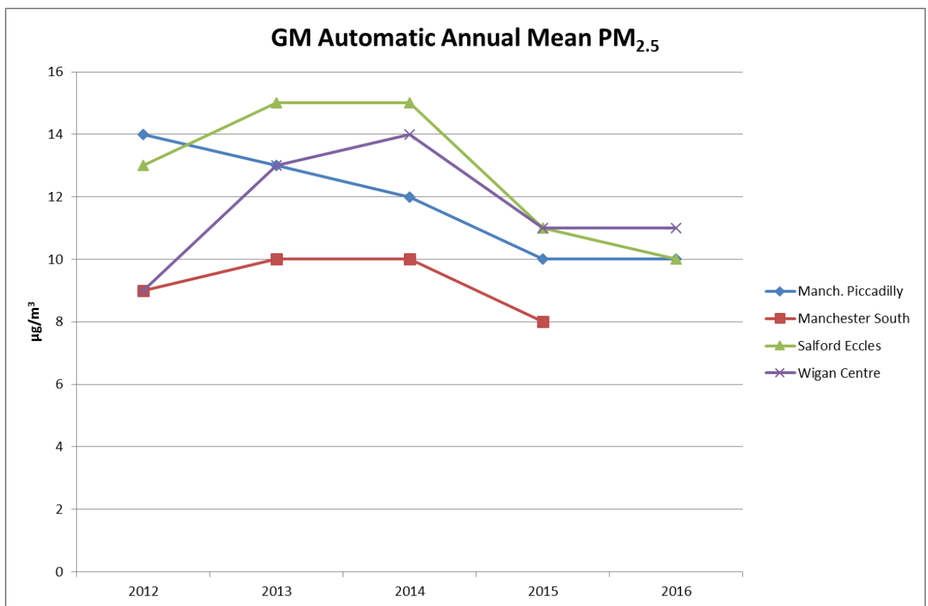
Figure 3.6 - Trends in Annual Mean PM 2.5 Concentrations Measured at Automatic Monitoring Sites
